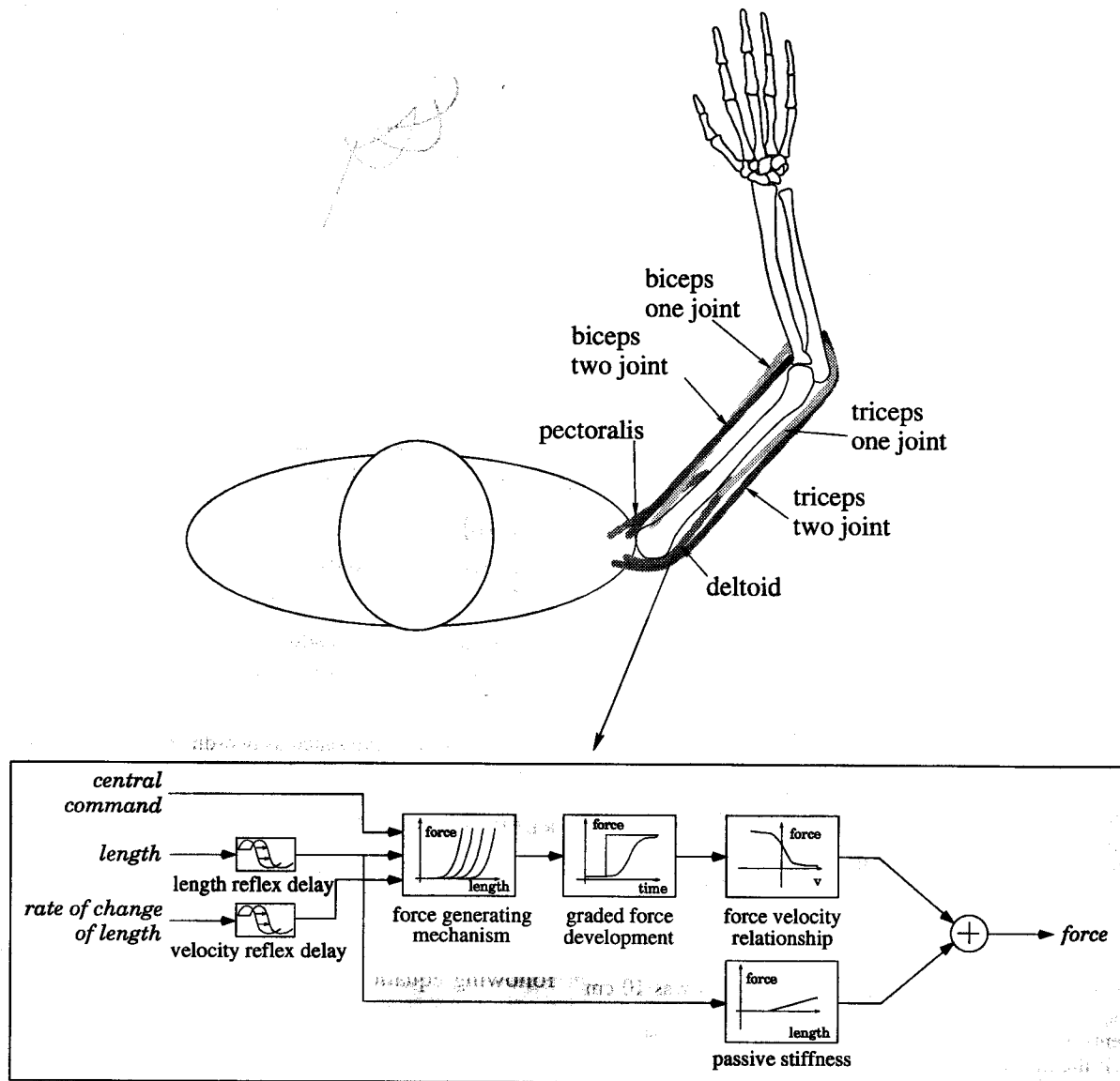
FIG. 1. Arm model. Six muscles are modeled, including 2 muscles that span both joints. Inset: schematic of the muscle model that includes the dependence of force on muscle length and velocity, the graded development of force over time, the passive elastic stiffness of muscle, and length and velocity afferent feedback with reflex delays.
