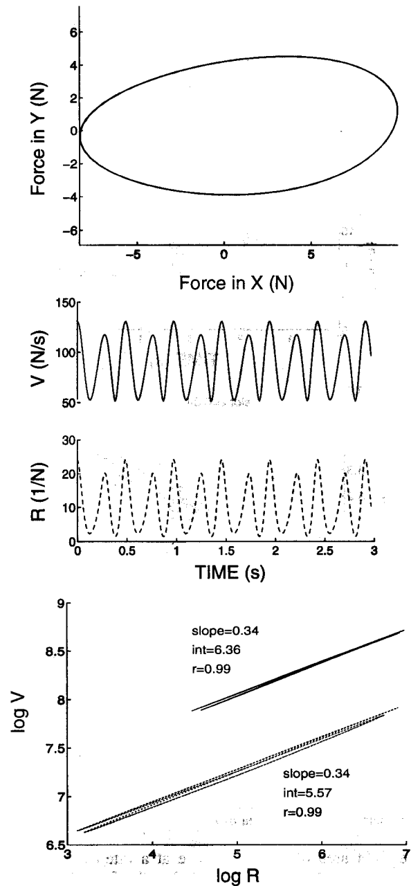
FIG. 5. Simulated elliptical force trajectories under isometric conditions. The hand was fixed in the center of the workspace, and forces at the hand were generated with the use of simulated control signals with constant tangential velocity. Top : simulated force trajectory at the hand generated by an elliptical equilibrium path shifted at a constant rate of 2.0 Hz. Middle : tangential velocity, V , and radius of curvature, R , plotted against time. Bottom : \log V plotted against \log R for elliptical force trajectories generated with the use of 2.0- and 1.5-Hz equilibrium shifts.
